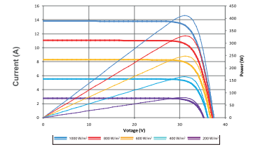
Current-Voltage & Power-Voltage Curve (410)
